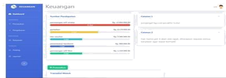
Gambar. 4.25 Halaman Pendapatan
